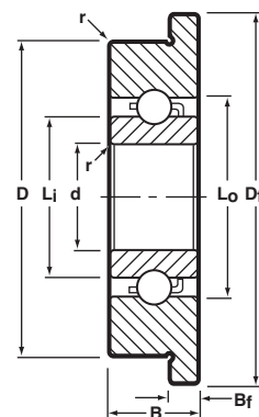
Flanged Crown Cage
