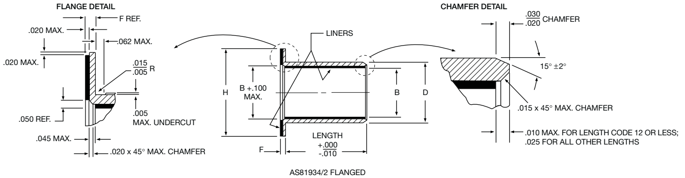
AS81934/2 FLANGED
